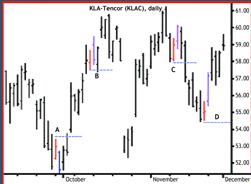
FIGURE 7 CONTINUATION PATTERNS
