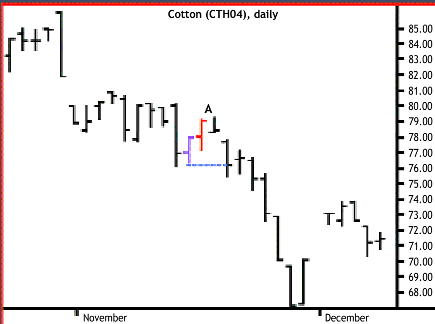
FIGURE 3 COMPACT HIKKAKES
